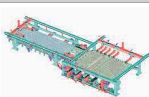
Rifilosquadratrice multilame Modul-LT / Modul-LT Trimming-squaring machine
